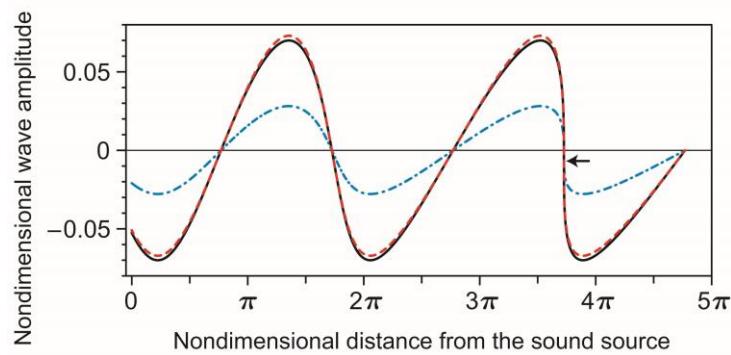
Figure 1 The nonlinear propagation of plane acoustic wave radiated by the sound source.
