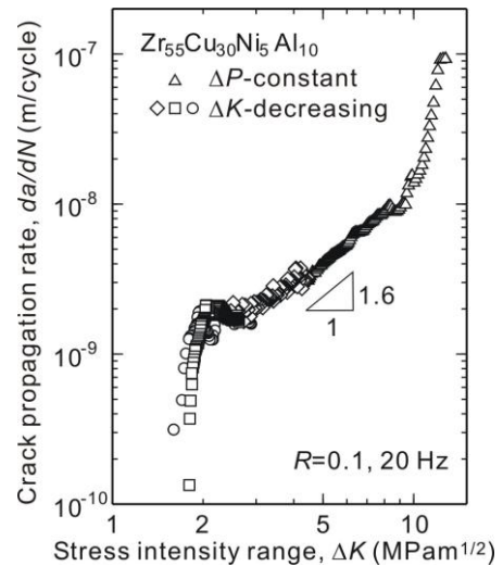
Fig. 1 Crack propagation behavior
