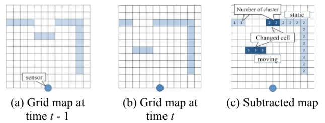
Fig. 1 Moving object detection
