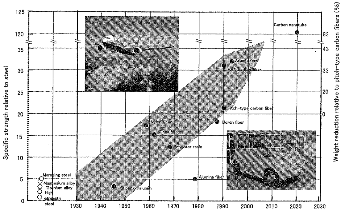
Fig.1 JSME Technological Roadmap for Specific Strength of Materials
