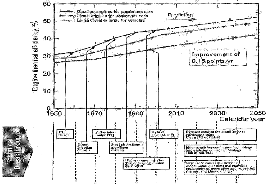
Fig.2 JSME Technological Roadmap for Thermal Efficiency of Engines
